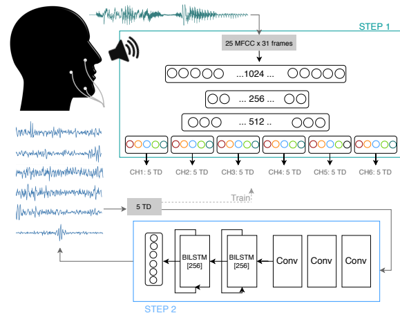
Figure 1: Two-step Speech-to-EMG system: Acoustic_{MFCC} -to- EMG_{TD} (step 1) followed by EMG_{TD} -to- EMG_{orig} (step 2).
